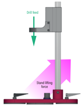
Fig. 2 Single column drill stand
